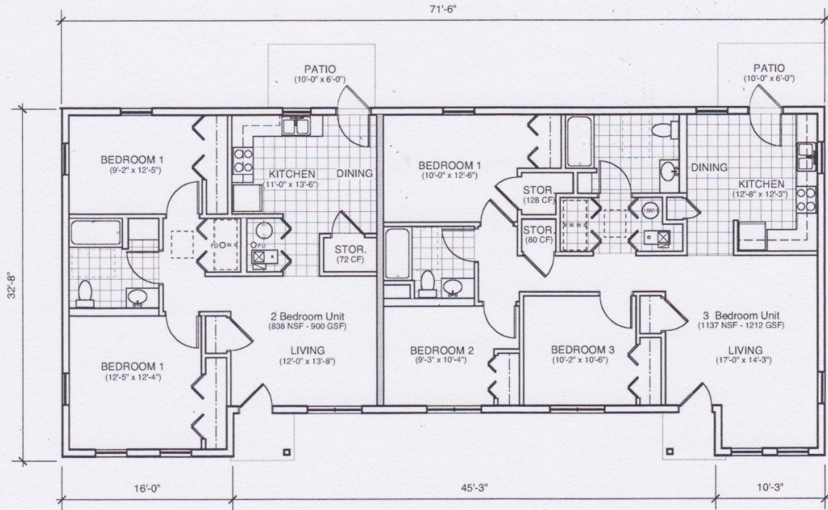
BUILDING TYPE C - (1) TWO BEDROOM UNIT & (1) THREE BEDROOM UNIT 1/8" = 1'-0"
